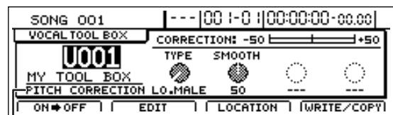
Algorithm name
